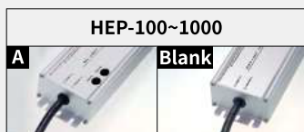
HEP-100 220x68x38.8 mm HEP-150/HEP-185 228x68x38.8 mm HEP-240 244.2x68x38.8 mm HEP-320 252x90x43.8 mm HEP-480 262x125x43.8 mm HEP-600 280x144x48.5 mm
